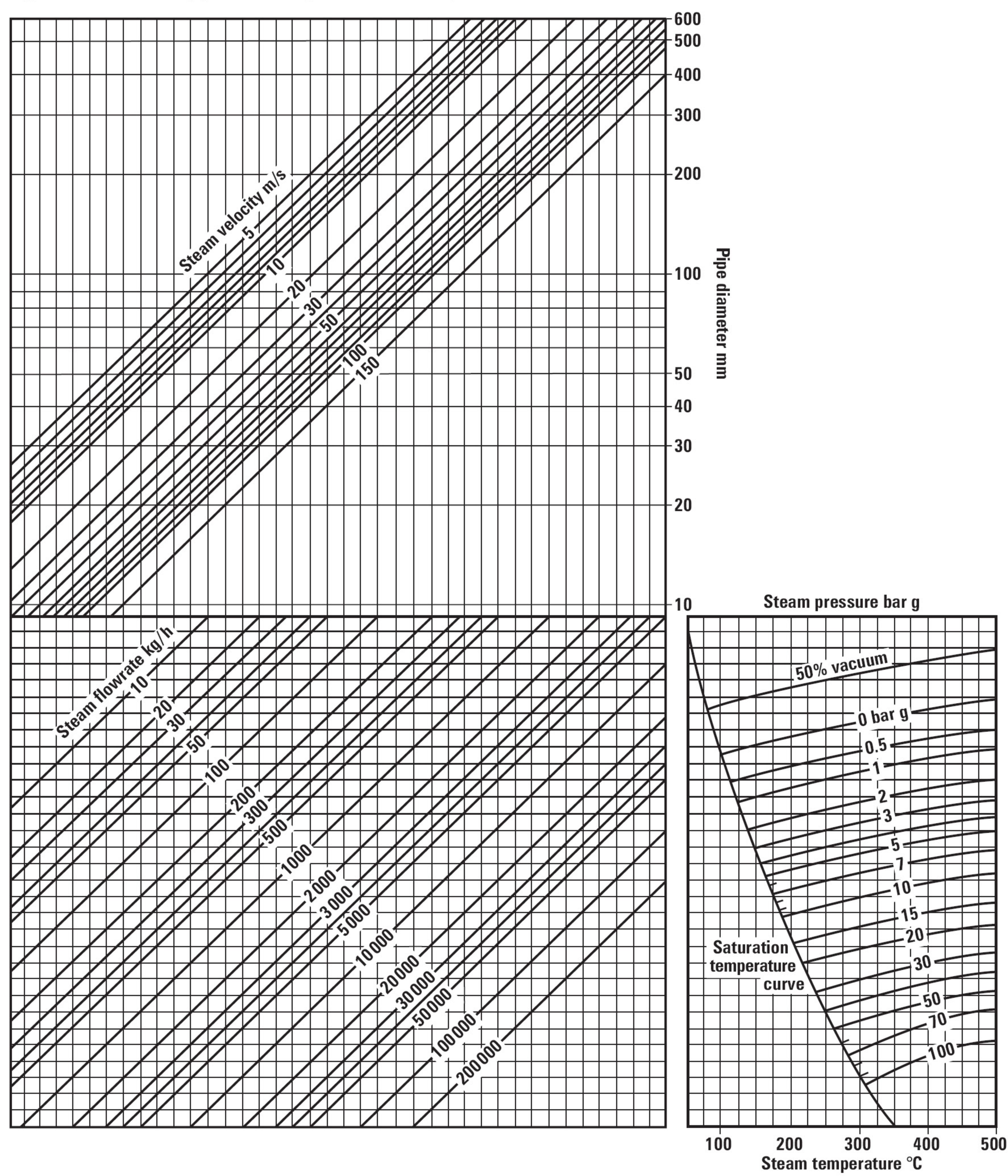
Fig. 10.2.10 Steam pipeline sizing chart - Velocity
